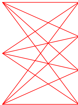
associations
