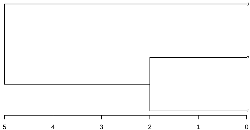
Host phylogeny
